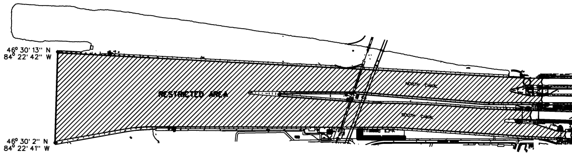
UPPER APPROACH PLAN
